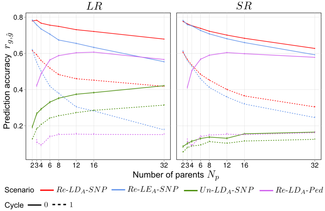
Figure S3 Average prediction accuracy r_{g,\hat{g}} in selection cycles C = 0 and C = 1 for synthetics produced from different numbers of parents N_p taken from ancestral populations SR and LR .
