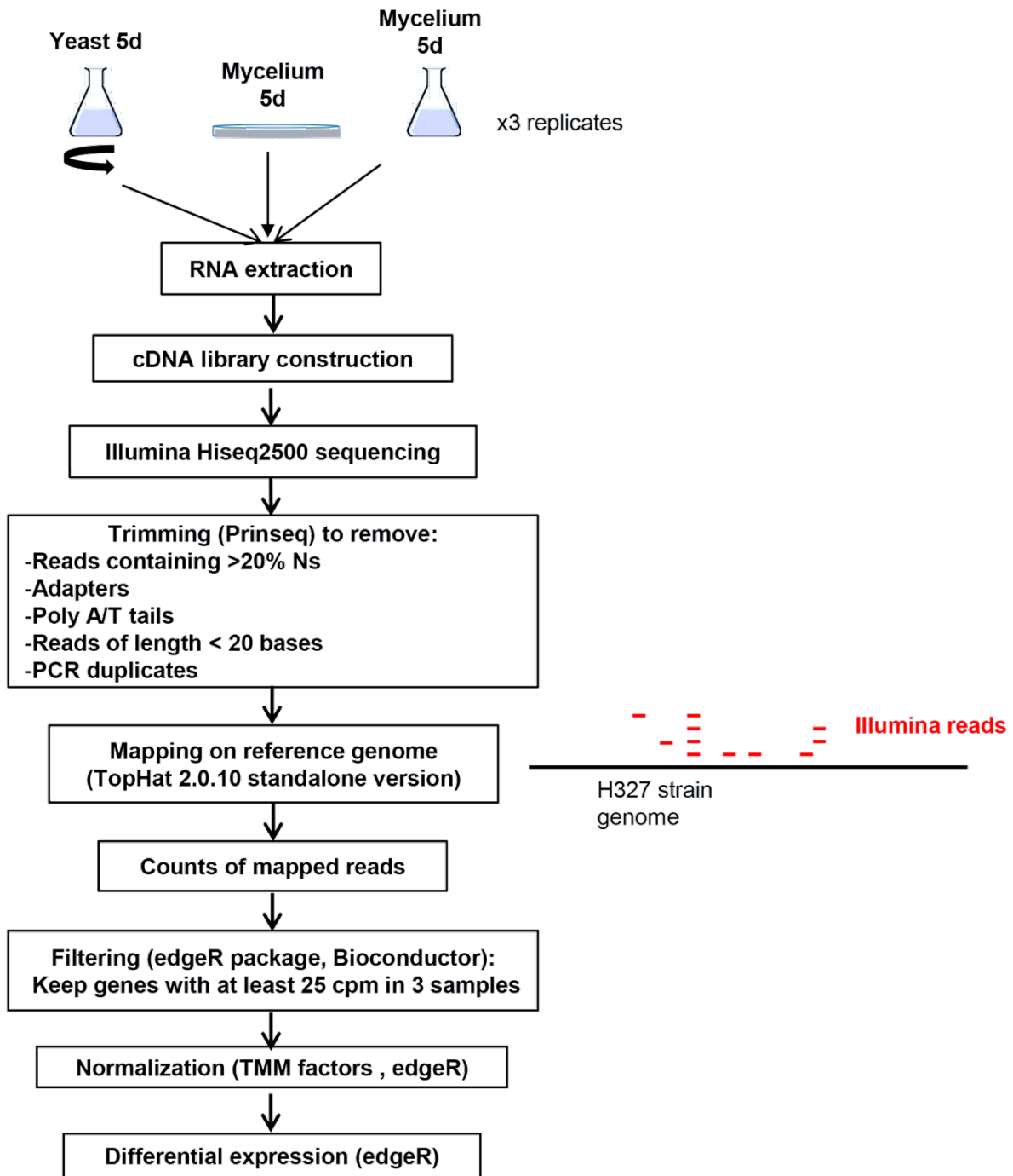
Figure S1 Workflow for RNAseq library preparation, cleaning and analysis for the three growth conditions (yeasts, mycelium on petri dishes and mycelium in flask, three replicates per condition) for Ophiostoma novo-ulmi .
