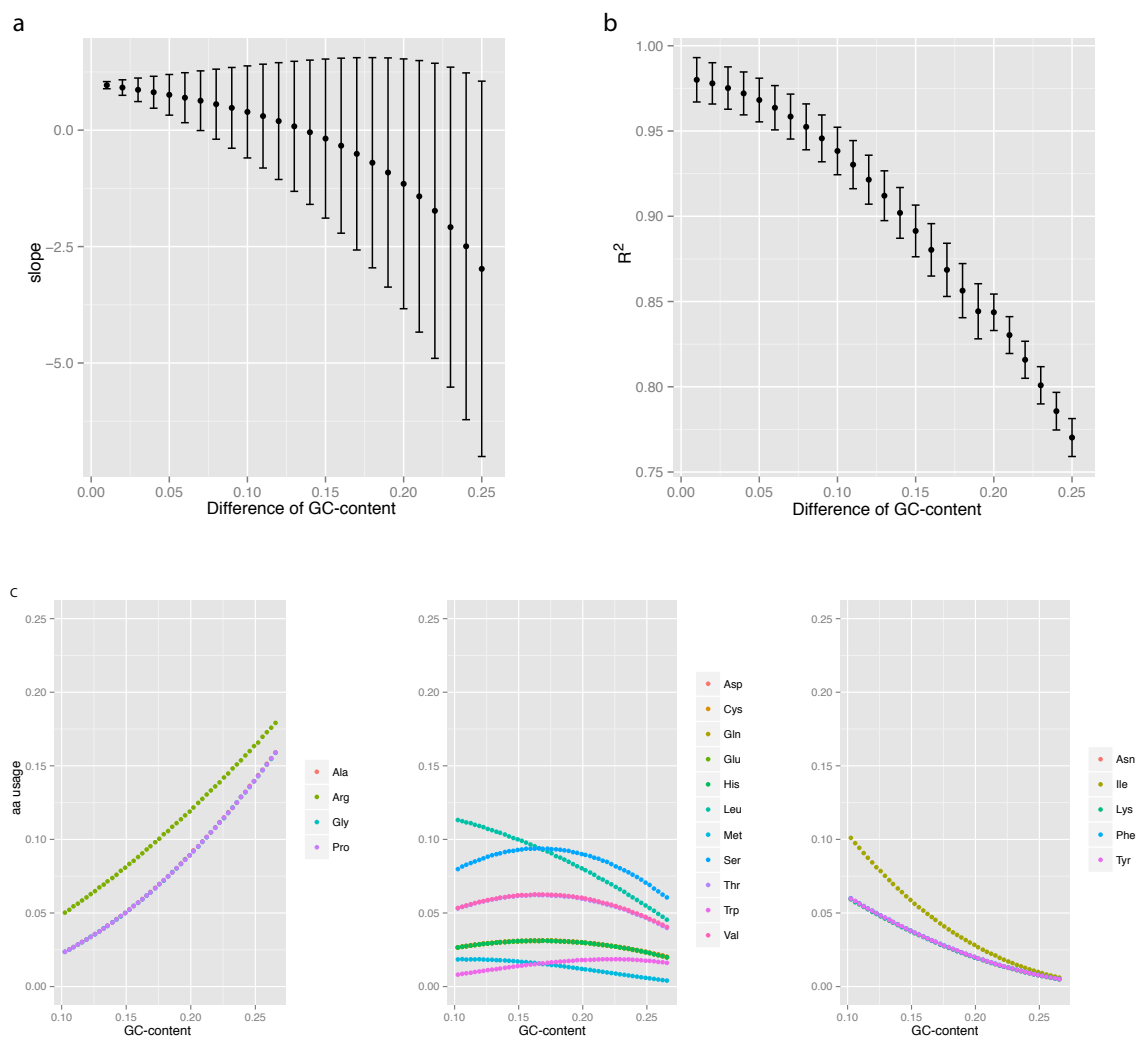
Figure S6. The patterns of the correlation slope (a) and the coefficient of determination R^2 values (b) for codon usages using simulated random sequences. (c) The usage frequency variation of amino acids in three groups along with the regional GC-content using simulated random sequences (Note that the curves of several amino acids are almost overlapped).
