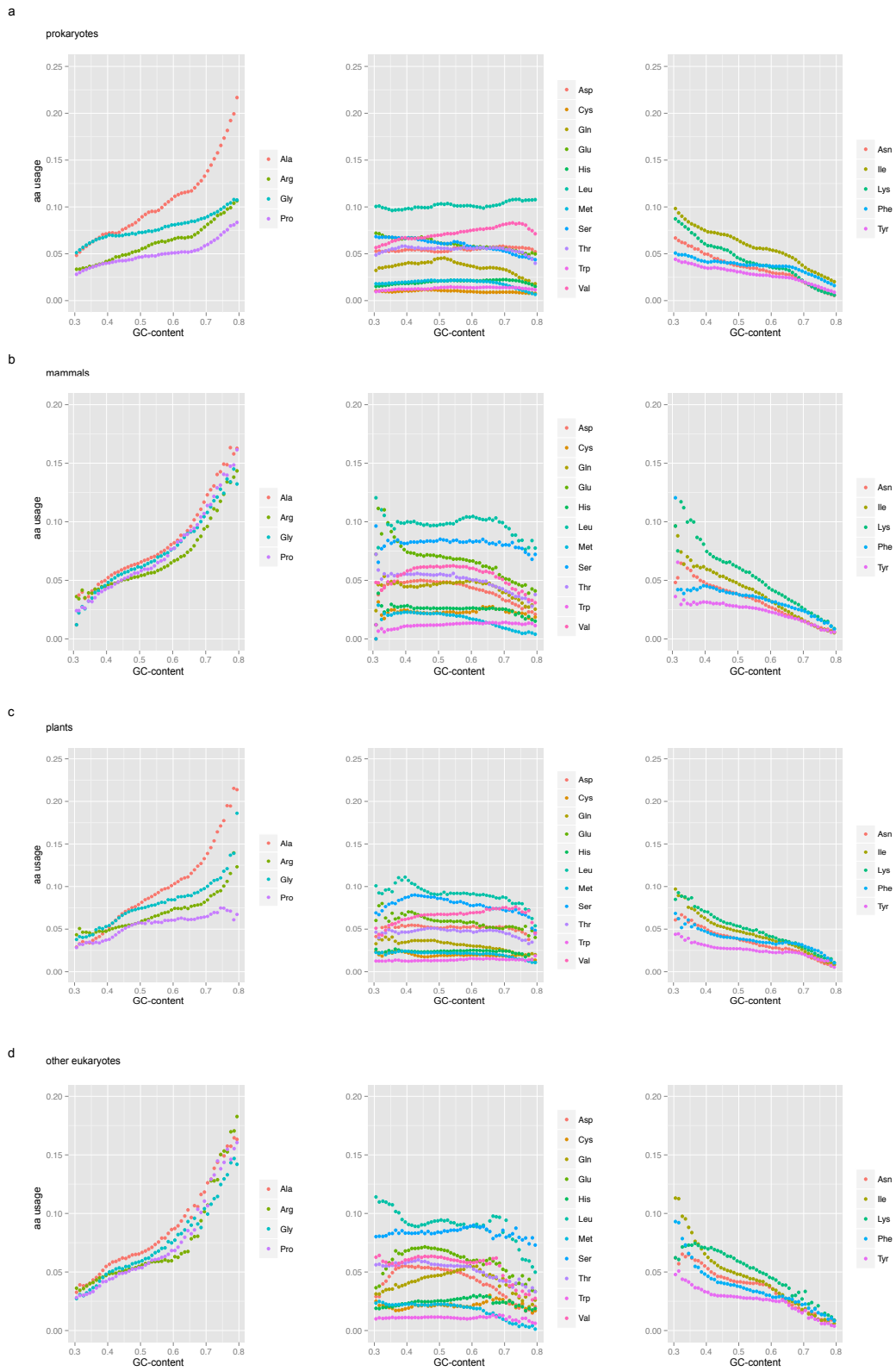
Figure S2. The usage frequency variation of amino acids in (a) prokaryotes, (b) mammals, (c) plants and (d) other eukaryotes along with the regional GC-content.
