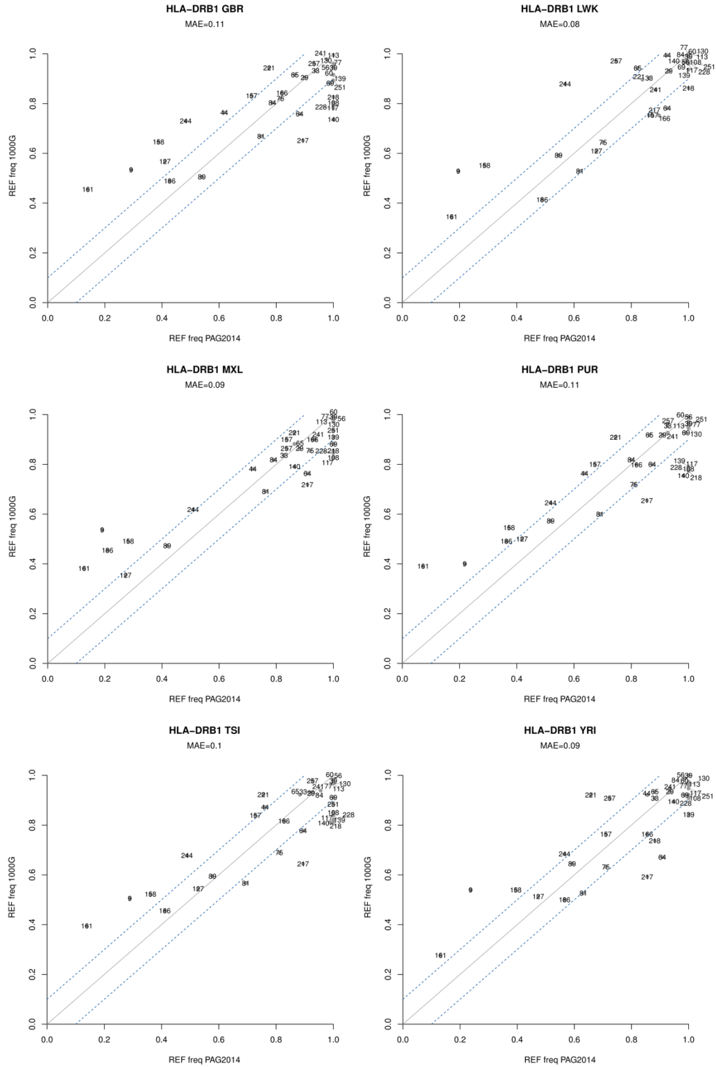
Figure S7 Reference allele frequency per population and per site in the HLA-DRB1 gene in the 1000 Genomes (1000G; y-axis) and Sanger sequencing (PAG2014; x-axis) datasets. Dashed lines indicate a \pm 0.1 deviation from the expected frequency (as estimated from PAG2014 dataset). MAE (mean absolute error) defined in Methods. Numbers indicate site position in ARS exons sequence.
