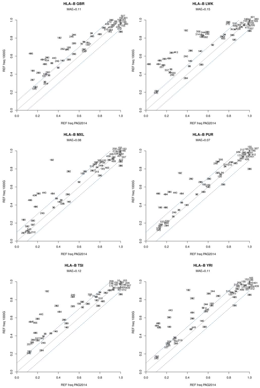
Figure S4 Reference allele frequency per population and per site in the HLA-B gene in the 1000 Genomes (1000G; y-axis) and Sanger sequencing (PAG2014; x-axis) datasets. Dashed lines indicate a \pm 0.1 deviation from the expected frequency (as estimated from PAG2014 dataset). MAE (mean absolute error) defined in Methods. Numbers indicate site position in ARS exons sequence.
