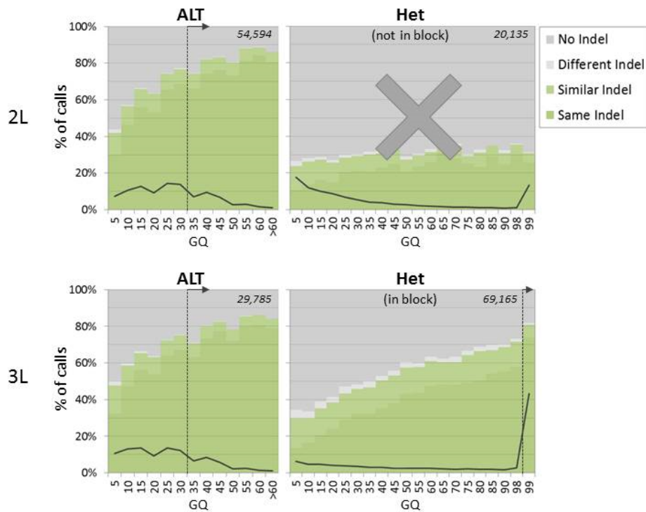
Figure S4 Small Indel Validation Rate Correlates with Genotype Quality Score
