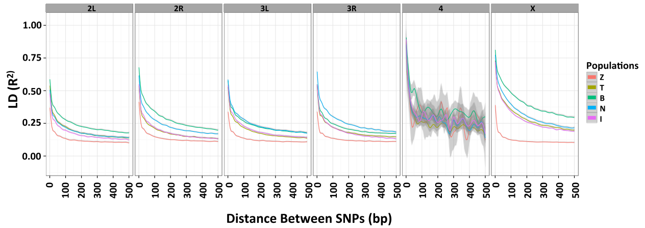
Figure S10 Decay of Linkage Disequilibrium Over Distance
