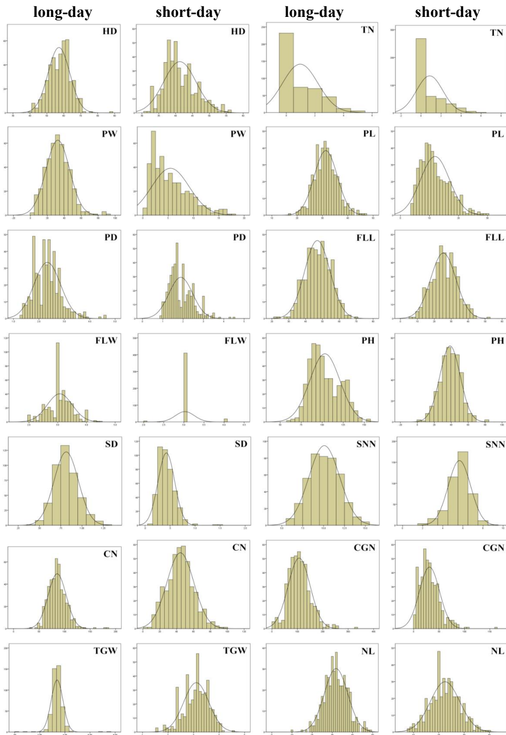
Figure S1 Distributions of the phenotypic data in the ‘zhang gu \times A2’ RIL population
