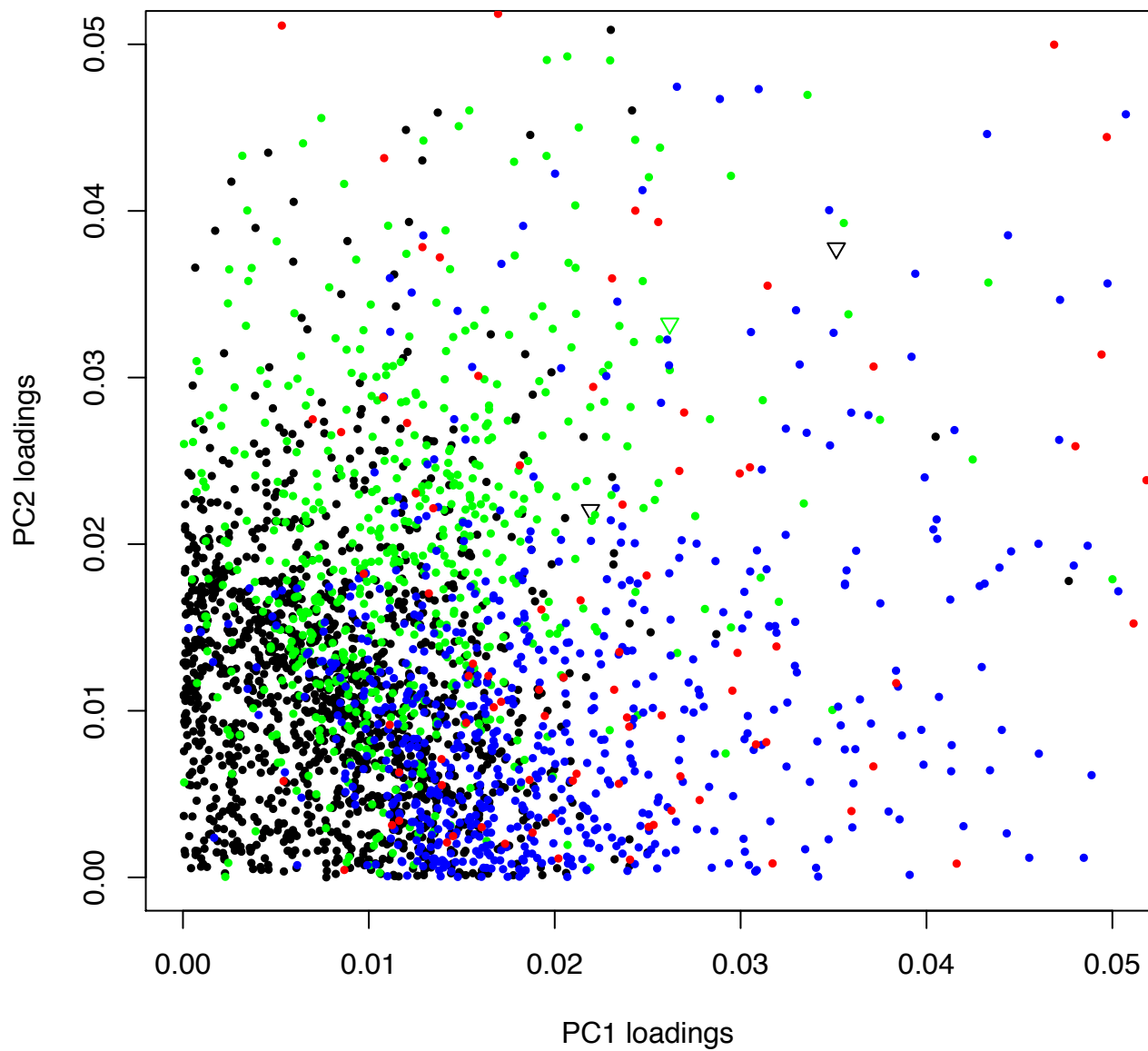
Figure S11B. This figure displays a zoomed-in version of the data in Figure S11A. Each axis scale is 0 to 0.05.
