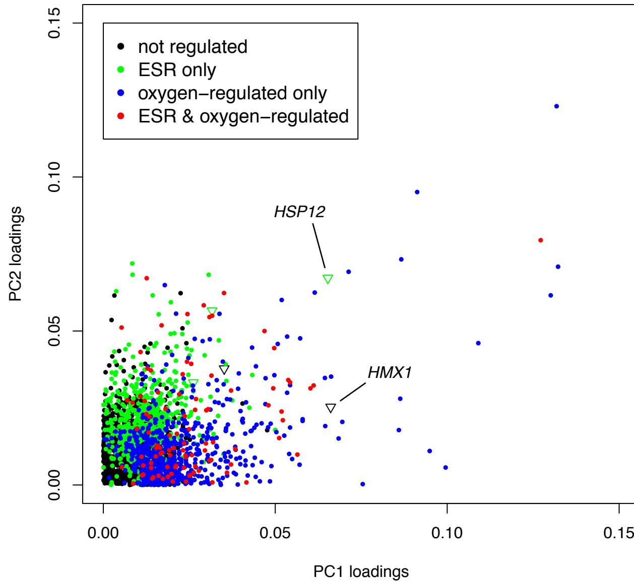
Figure S11A. The PC1 and PC2 loadings for all genes following PCA. Each data point is a gene. The six triangles represent genes that are discussed in the text and the triangles are color coded as in the legend.
