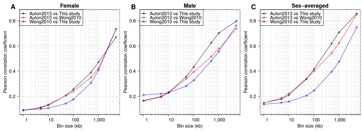
Figure S8: Pearson correlation between recombination rates estimated from the Auton et al. 1 LD map, the pedigree maps from Wong et al. 2 , and this study as a function of scale.
