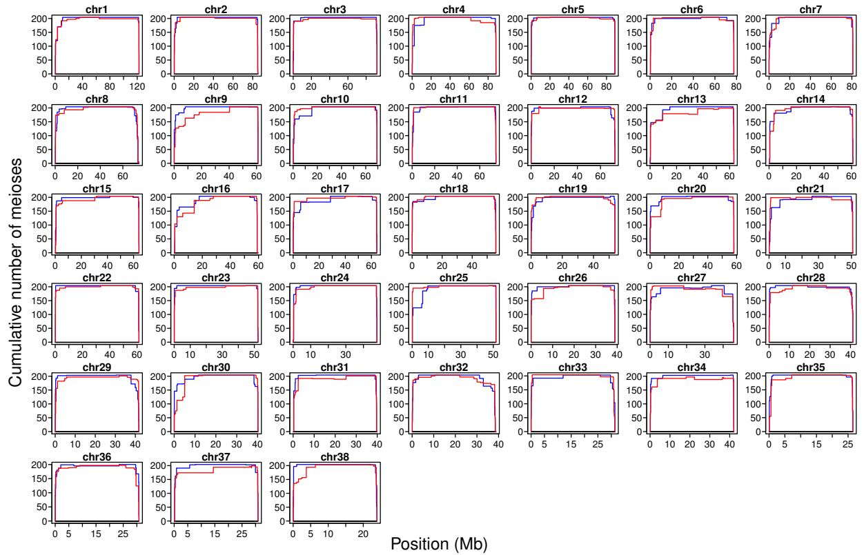
Figure S4: The effective number of meioses as a function of physical position is shown along each chromosome. Red curves represent females ( n=204 ), blue curves represent males ( n=204 ).
