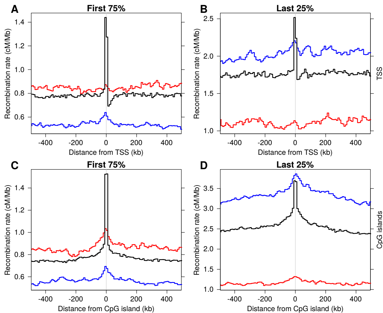
Figure S14: Recombination around TSS and CpG islands partitioned by chromosome position. Male rates are in blue, female in red, rates from the LD map in black. Rates were estimated in 10 kb bins. Rates were estimated for each feature by taking the centromeric 75% (A and C) and telomeric 25% (B and D) of each chromosome separately.
