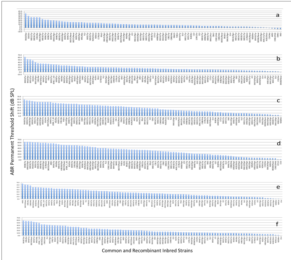
Figure S1. ABR permanent threshold shift at 4kHz (a), 8 kHz (b), 12 kHz (c), 16 kHz (d), 24 kHz (e) and 32 kHz (f) tone burst in 100 HMDP inbred strains.
