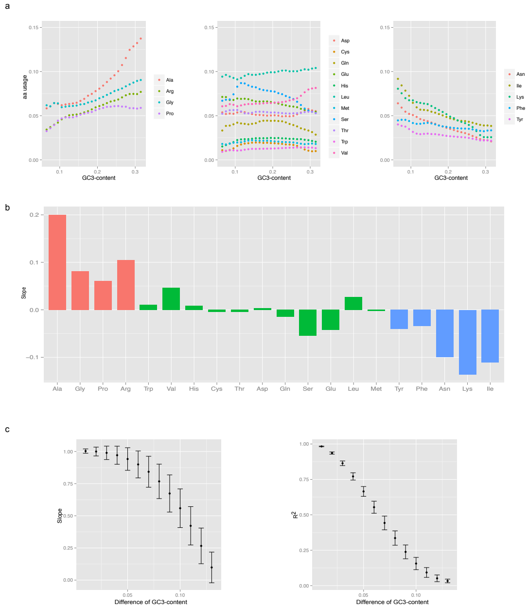
Figure S4. Codon and amino acid usage with GC3-content. (a) The usage frequency variation of amino acids in three groups along with the regional GC3-content; (b) the slope value in a linear regression analysis for the lines in (a); (c) The patterns of the correlation slope (left) and the coefficient of determination R^2 values (right) for codon usages between different GC3-groups.
