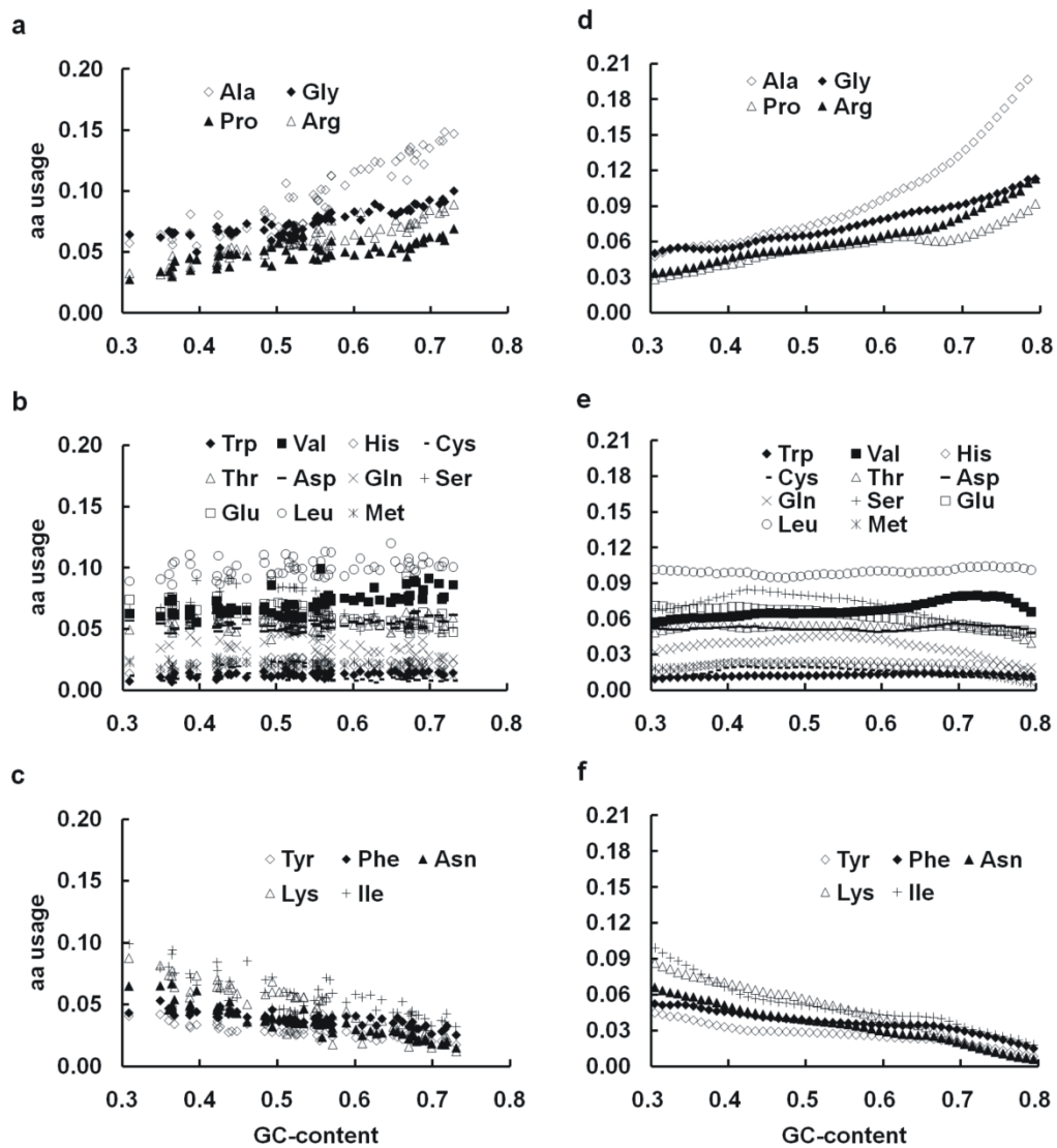
Figure S1 Patterns of amino acid usages when species (a-c) and CDSs (d-f) were used as analysis units. Three types (a-c or d-f) of amino acids based upon GC_{syn} change differently as the GC-content increases.
