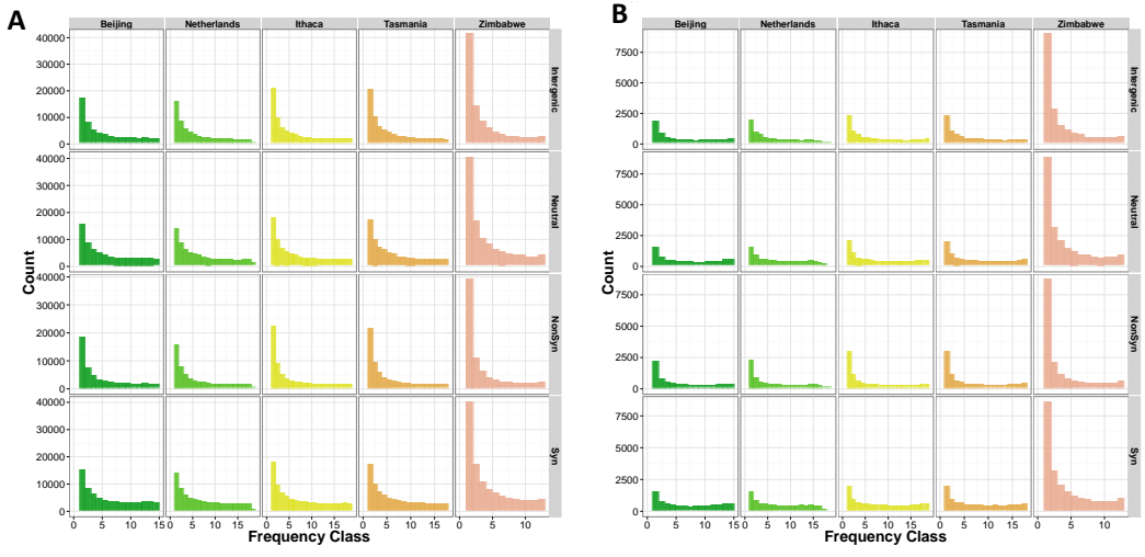
Figure S9 Population-Specific Site Frequency Spectra for Four Classes of SNPs
