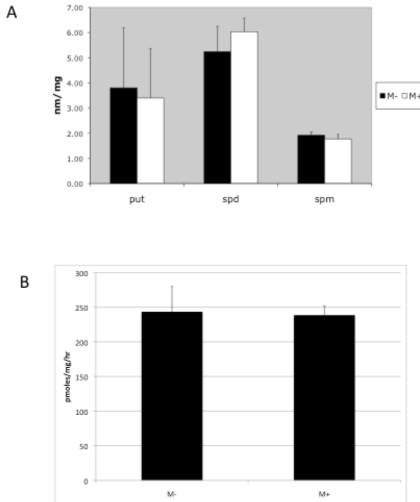
Figure S3 Polyamine and ODC activity of MTAP+ and MTAP- cells. A. Intracellular concentration of putrescine, spermidine, and spermine. Error bars show standard deviation (n=3). B. ODC activity. Error bars show standard deviation (n=3).
