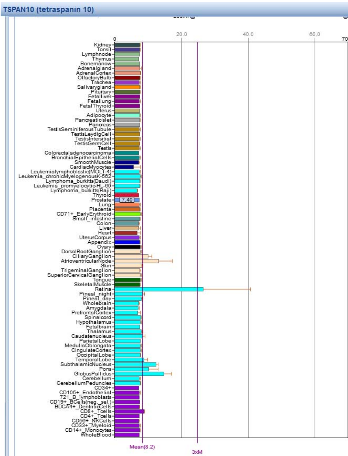
Figure displaying BioGPS normalized tissue expression for the gene TSPAN10, highly biased in M. lucifugus .
