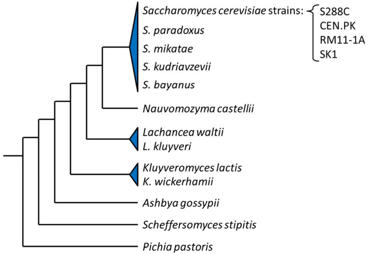
Figure S1 M-Y species phylogeny. Phylogenetic tree of the 16 Ascomycetes yeast strains used in the M-Y sample (Table S1).
