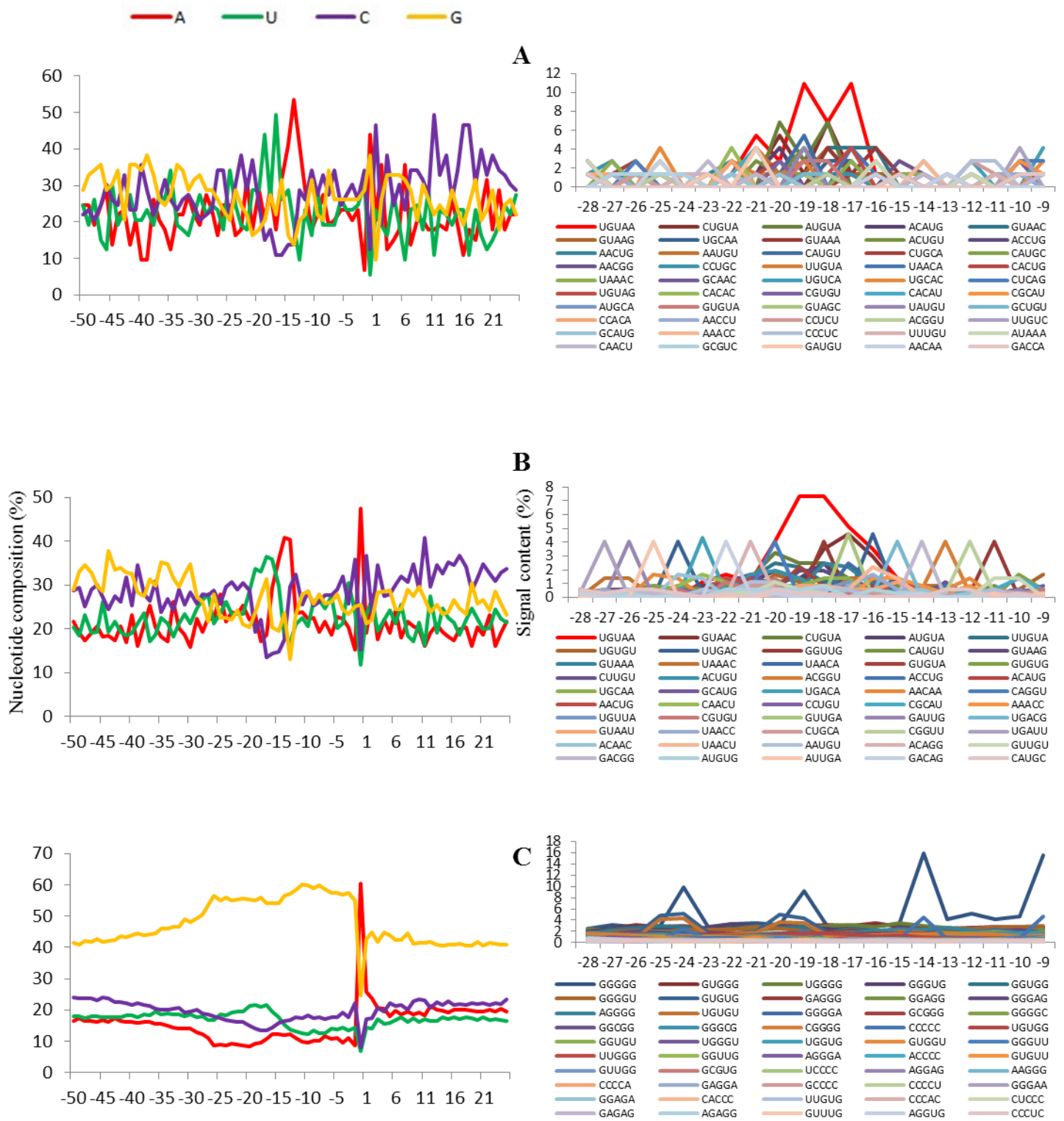
Figure S7 The single nucleotide profiles (-50 to +25) and top frequent motifs in NUE regions (-28 to -5) of poly(A) sites in intron from different PAC datasets. (A) EST data. (B) 454 data. (C) Illumina data.
