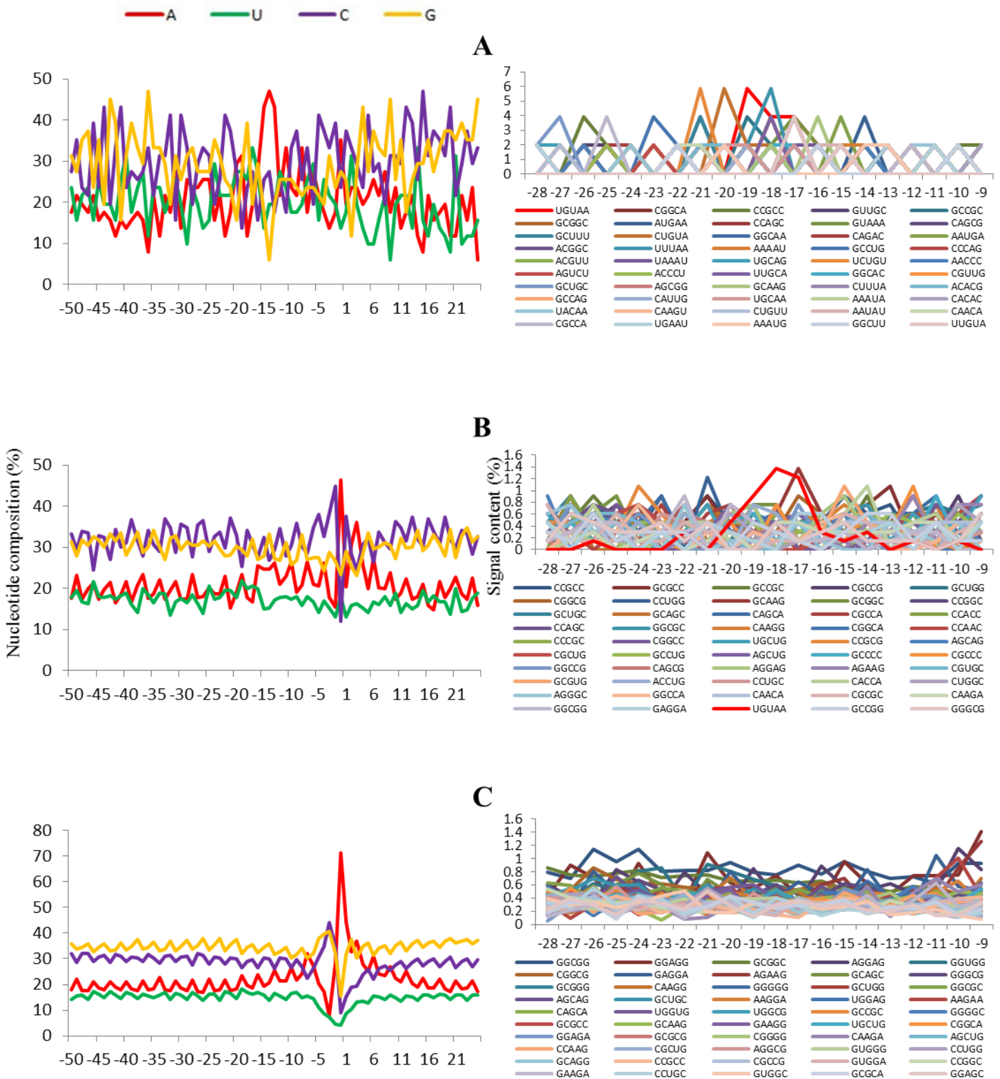
Figure S6 The single nucleotide profiles (-50 to +25) and top frequent motifs in NUE regions (-28 to -5) of poly(A) sites in CDS from different PAC datasets. (A) EST data. (B) 454 data. (C) Illumina data.
