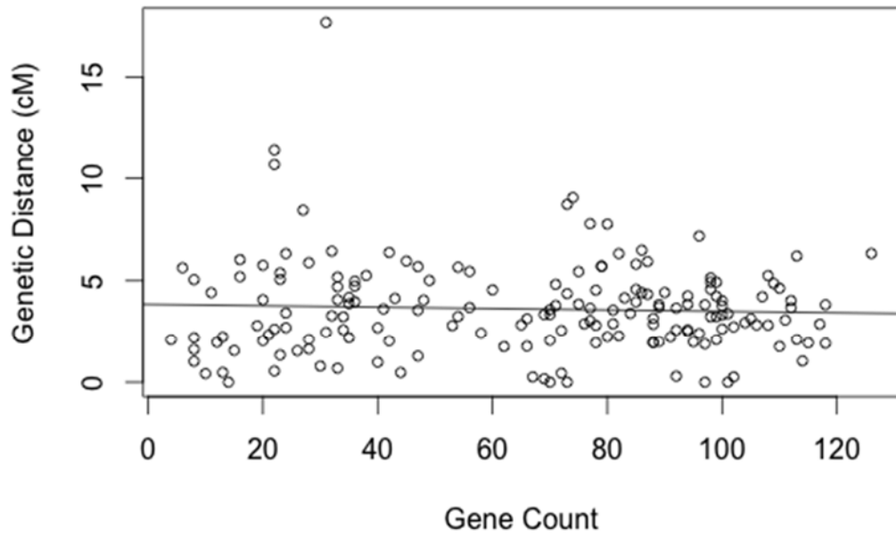
Figure S2 The number of genes plotted against the genetic distance for windows of ~500 kb. Only scaffolds >500 kb were included in the figure. The solid line is a least squares regression line indicating little evidence of a relationship.
