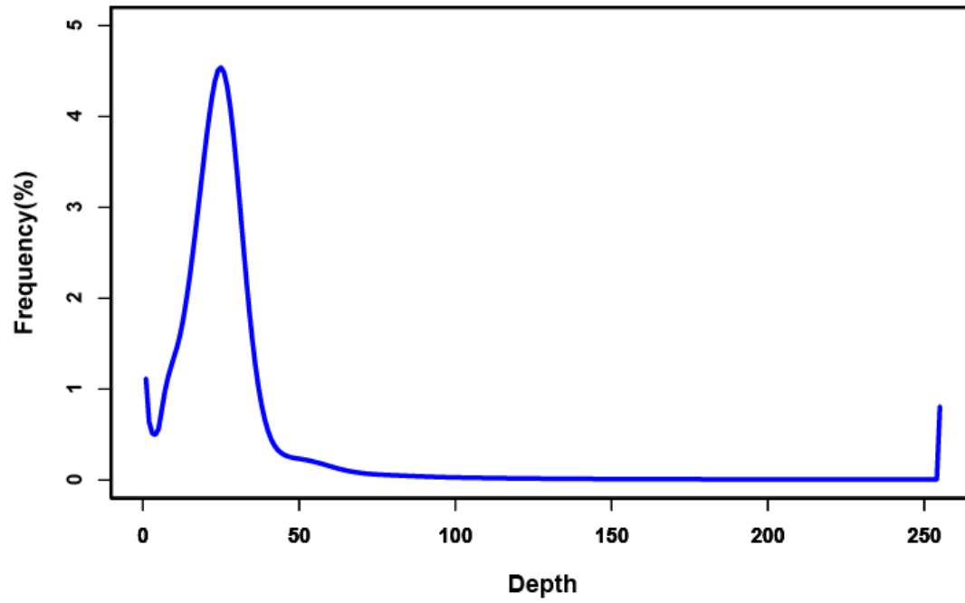
Figure S1 17-kmer estimation of genome size. The genome size of Drosophila suzukii was estimated to be 220Mb based on reads from short insert size libraries.
