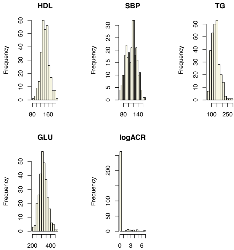
Figure S3 The distribution of the trait values.
