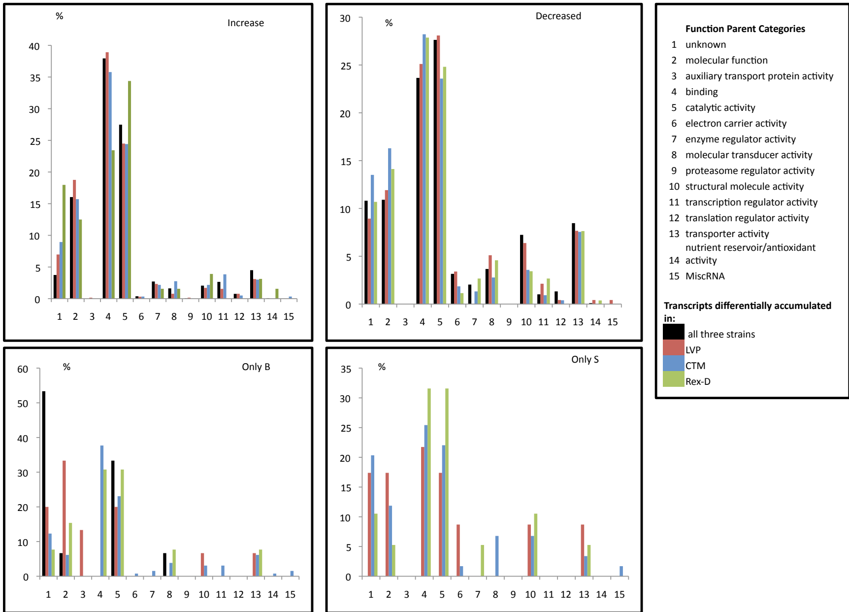
Figure S6 Function parent of differentially-accumulated transcripts. Function parent attribution of the transcripts accumulated differentially at 5 hPBM mosquitoes of the LVP, CTM and Rex-D strains.
