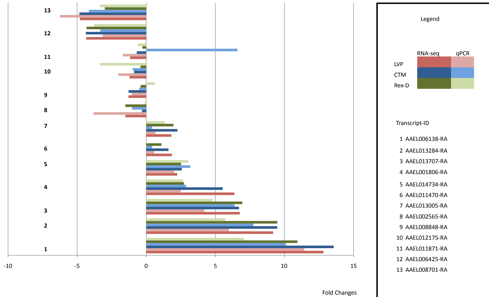
Figure S2 RNA-seq data validation by qRT-PCR. Average fold-changes detected between S and B Aedes aegypti mosquitoes of the LVP, CTM and Rex-D strains by RNA-seq and qRT-PCR on a random selection of thirteen genes.
