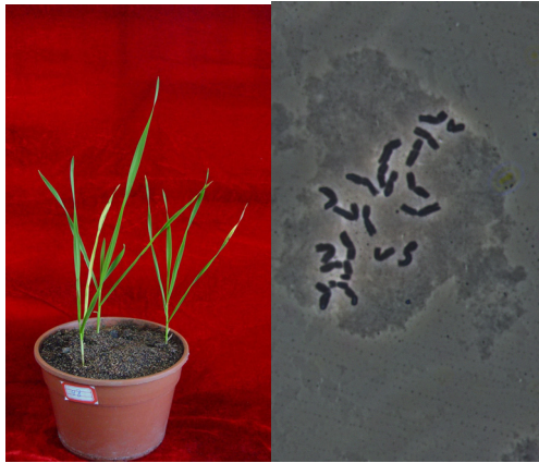
Figure S1 Karyotype analysis in root tips of the haploid wheat. Cytological preparations were carried out on root tips obtained from seeds germinated on sterile moist filter paper in Petri dishes at 25°C. Roots were pretreated with 0.05% colchicine solution for 2–3 h. and fixed in Carnoy for 24 h. and stored in 70% ethanol at 4°C.
