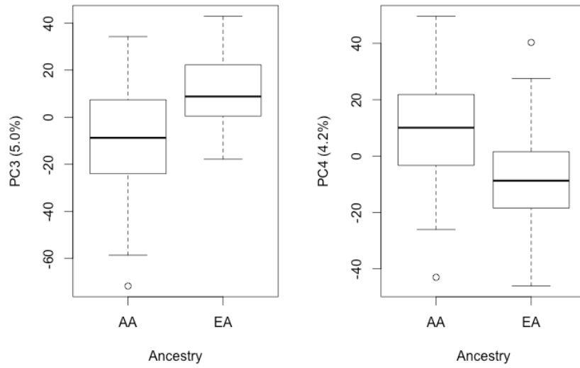
Figure S4: Boxplot showing inter-ethnic variation in covariates-corrected expression data captured by PC3 and PC4, with the proportion of variation explained in parenthesis.
