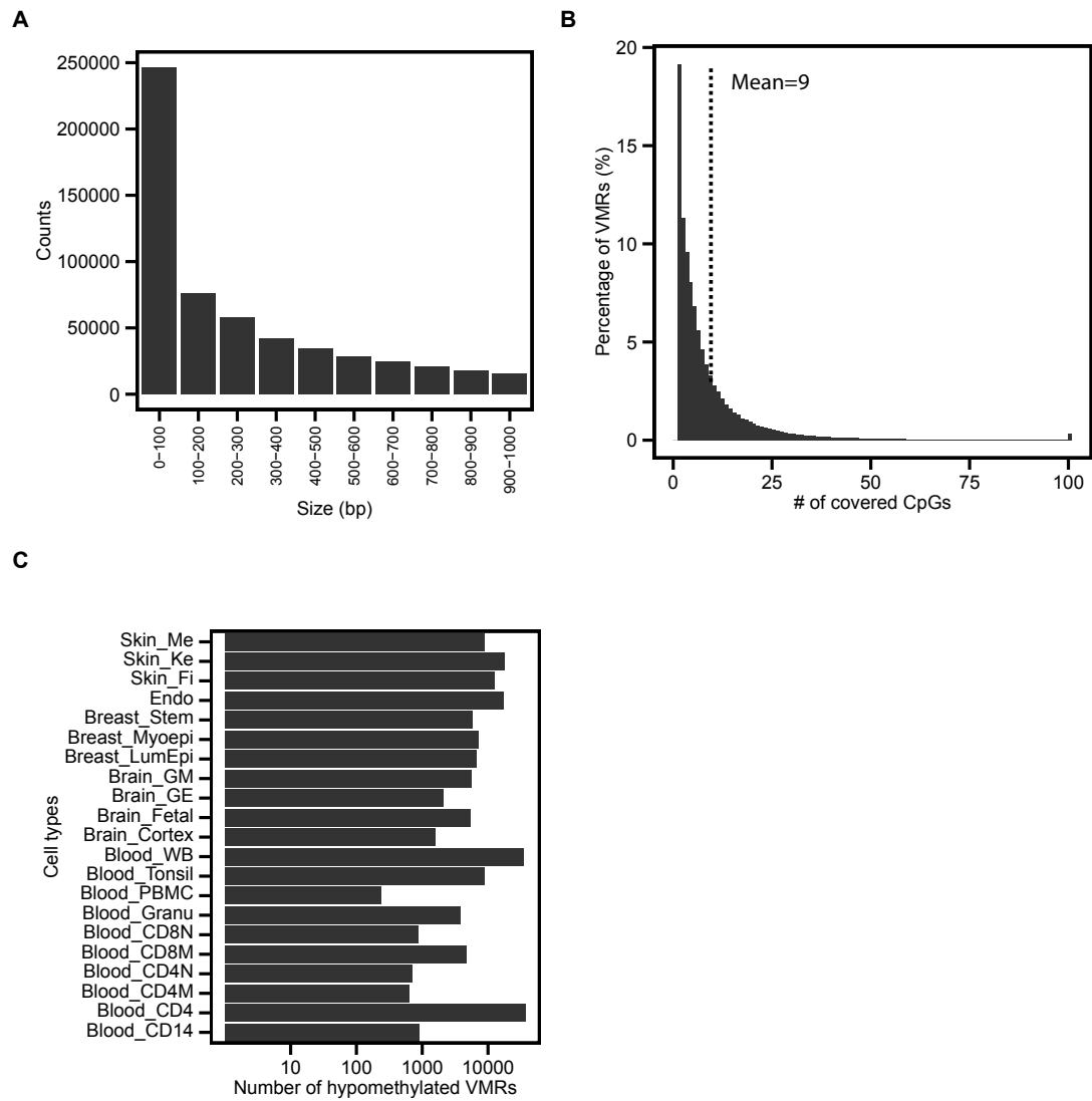
Figure S4. Characterization of variably methylated regions (VMRs) continued.
