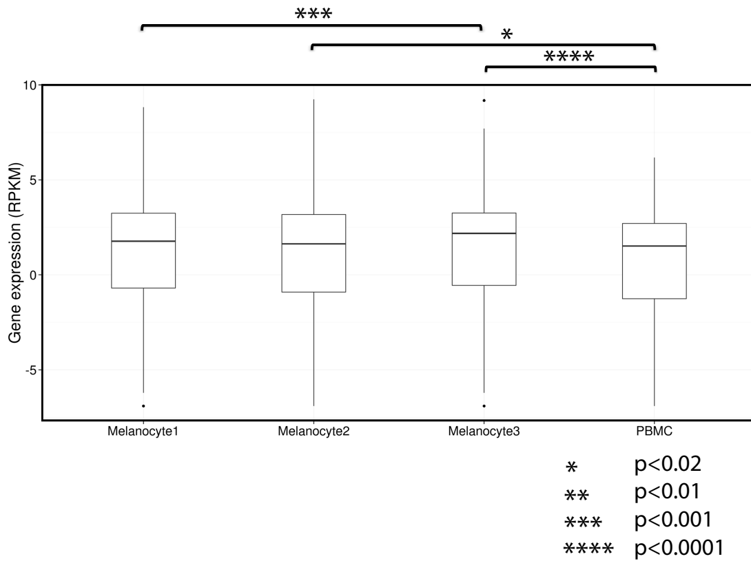
Figure S13. Genes near hypomethylated VMRs show increased expression. RNA-seq derived expression values of genes within 10kb regions of melanocyte hypomethylated VMRs were calculated for melanocyte and PBMC and Kruskal-Wallis test was used to compare expression levels between samples.
