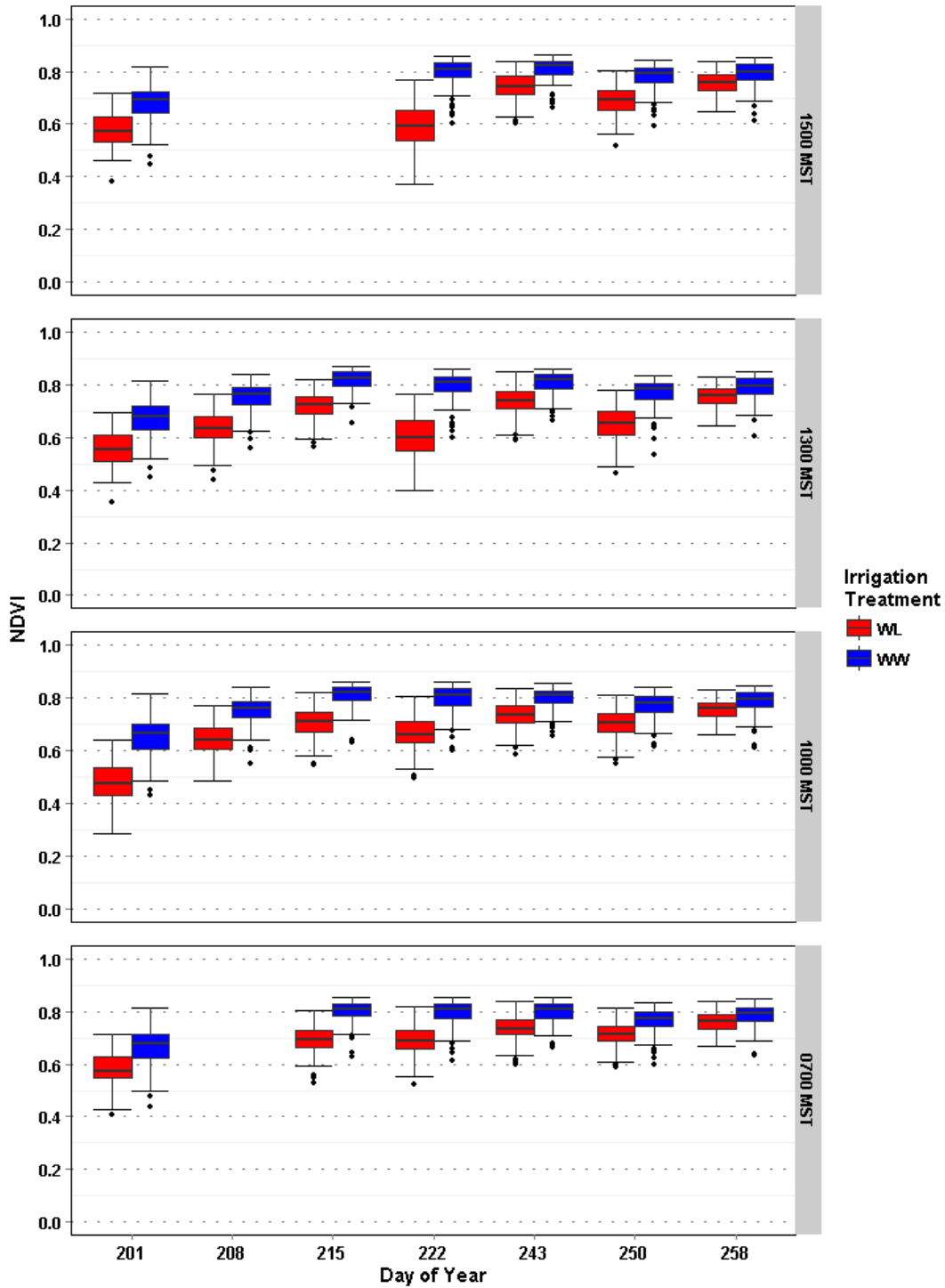
Figure S9 Box-and-whisker plots of best linear unbiased estimators (BLUES) for normalized difference vegetation index (NDVI; unitless) collected from the TM-1×NM24016 mapping population and its parents for the 2012 growing season under two irrigation regimes, water-limited (WL) and well-watered (WW). The horizontal black line inside the box is the median.
