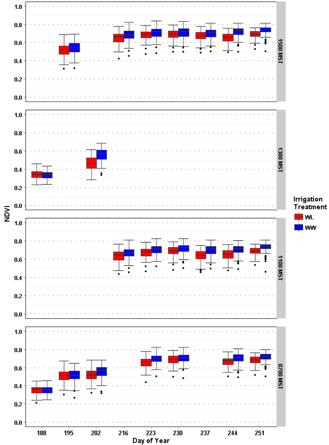
Figure S8 Box-and-whisker plots of best linear unbiased estimators (BLUEs) for normalized difference vegetation index (NDVI; unitless) collected from the TM-1×NM24016 mapping population and its parents for the 2011 growing season under two irrigation regimes, water-limited (WL) and well-watered (WW). The horizontal black line inside the box is the median.
