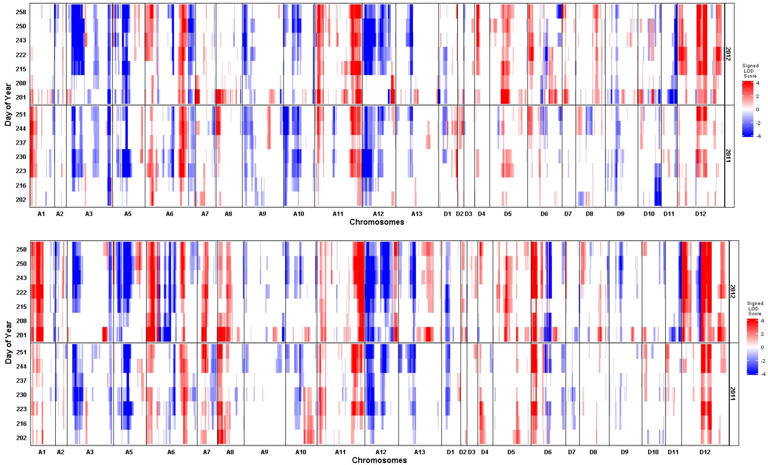
Figure S27 Genome-wide scan for quantitative trait loci (QTL) associated with leaf area index (LAI) across two years under two irrigation regimes, water-limited (WL, top panel) and well-watered (WW, bottom panel). Color is representative of the estimated additive allelic effect, with red and blue colors indicating increased and decreased LAI, respectively, when substituting a NM24016 allele with an allele from TM-1. The intensity of the color represents the magnitude of the logarithm of odds (LOD) score with 3.3 as the significance threshold to declare QTL – values above 3.3 were assigned a value of 4 for presentation purposes. The left-hand y-axis denotes day of the growing season (Julian calendar) that data were collected, and the right-hand y-axis denotes year. The x-axis represents the mapped chromosomes of tetraploid cotton with marker intervals in centimorgans (cM). Chromosomes A04 and D13 did not have any mapped markers.
