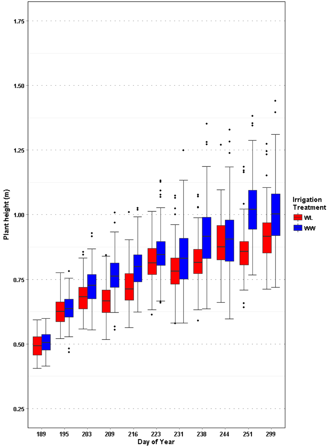
Figure S22 Box-and-whisker plots of best linear unbiased estimators (BLUEs) for plant height (m) collected from the TM-1xNM24016 mapping population and its parents for the 2011 growing season under two irrigation regimes, water-limited (WL) and well-watered (WW). The horizontal black line inside the box is the median.
