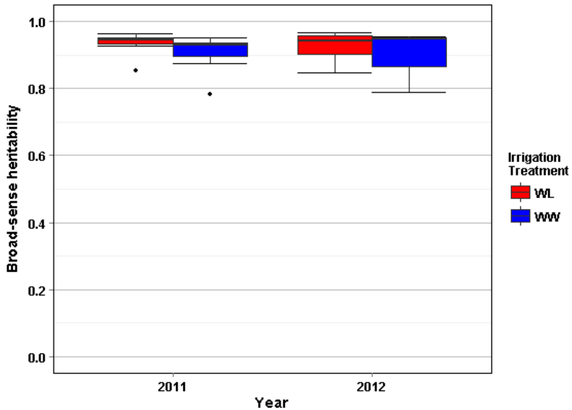
Figure S18 Box-and-whisker plots of estimates of broad-sense heritability ( \hat{H}^2 ) on an entry-mean basis for canopy height across two years under two irrigation regimes, water-limited (WL) and well-watered (WW). The total number of times that the high-throughput plant phenotyping (HTPP) system was driven over the entire set of experimental plots to collect canopy height data was 18 and 22 for 2011 and 2012, respectively. The horizontal black line inside the box is the median.
