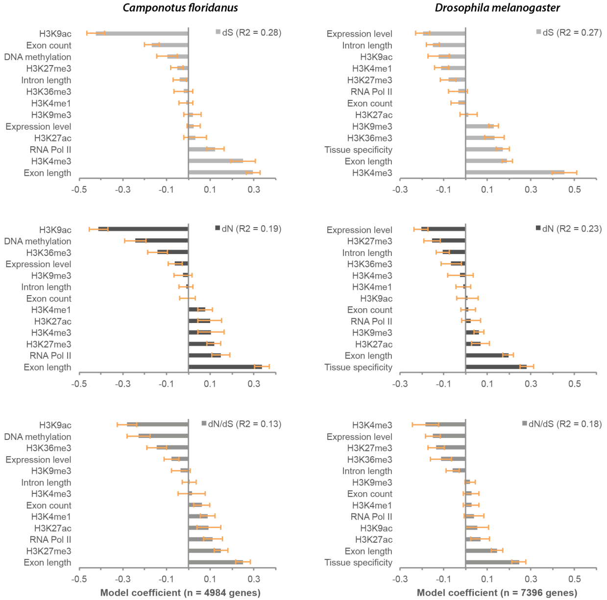
Figure S2. Relationship between sequence substitution rate and gene characteristics according to multiple linear regression models in the ant C. floridanus and the fly D. melanogaster . Model coefficients are plotted with 95% confidence intervals.
