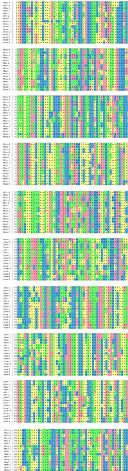
Figure S3 (Related to Figure 2): Nucleotide sequence alignment of mtrA domain in Methanomicrobiales.
