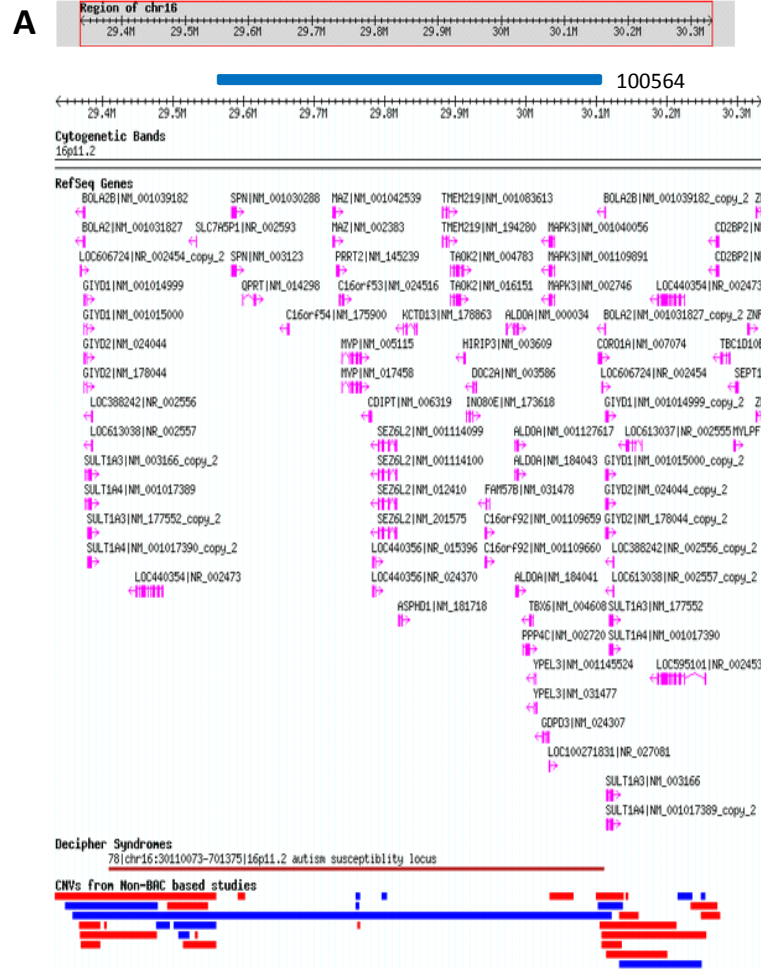
Figure S2 (A) Genome browser view of 16p11.2 duplication (B) Genome browser view of 22q11.22-q11.23 duplication region
