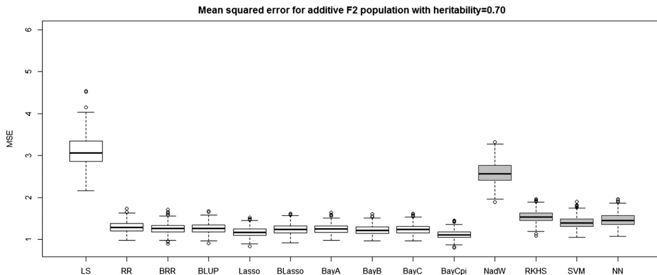
Figure 9 The boxplots of mean squared error for the F_2 population with additive genetic architecture and heritability of 0.70. The first 10 boxplots correspond to the parametric methods, and the last four (gray) boxplots correspond to the nonparametric methods.
