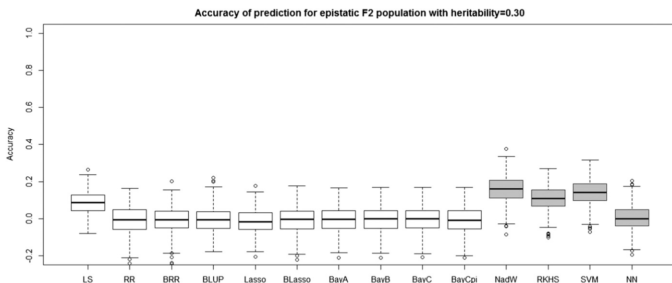
Figure 8 The boxplots of accuracy of prediction for the F_2 population with epistatic genetic architecture and heritability of 0.30. The first 10 boxplots correspond to the parametric methods, and the last four (gray) boxplots correspond to the nonparametric methods.
