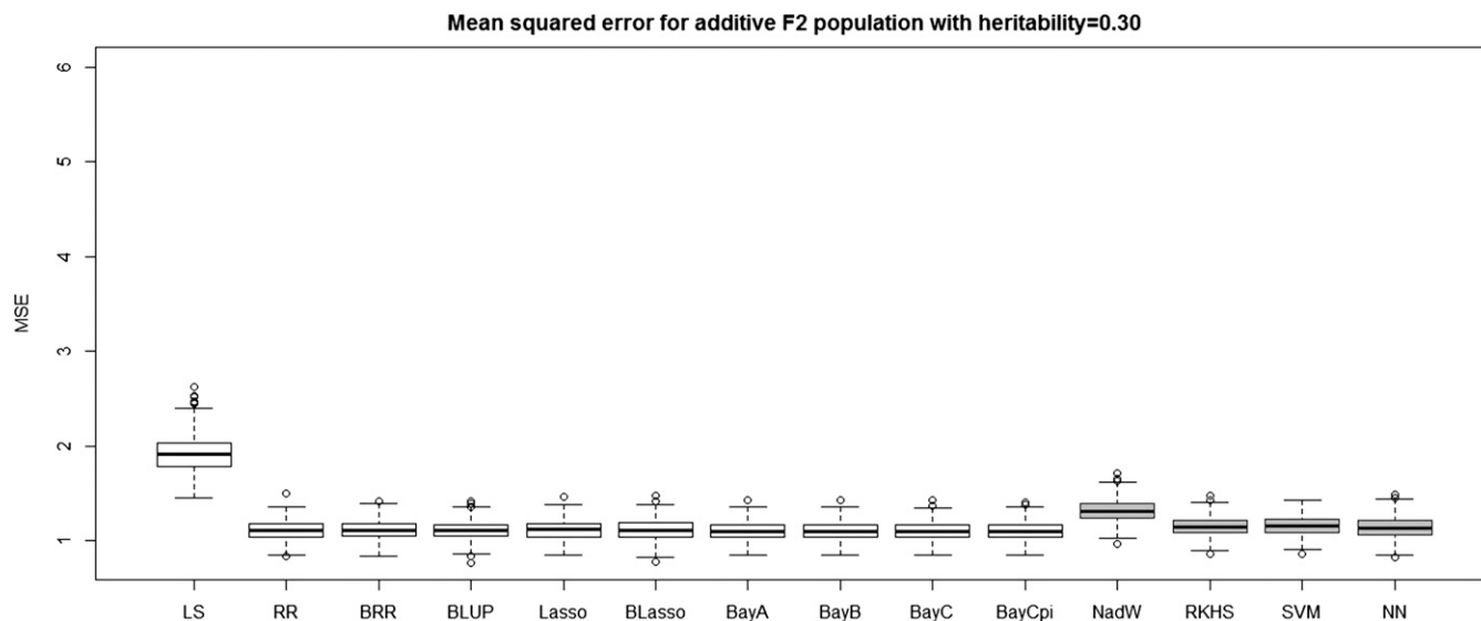
Figure 11 The boxplots of mean squared error for the F_2 population with additive genetic architecture and heritability of 0.30. The first 10 boxplots correspond to the parametric methods, and the last four (gray) boxplots correspond to the nonparametric methods.
