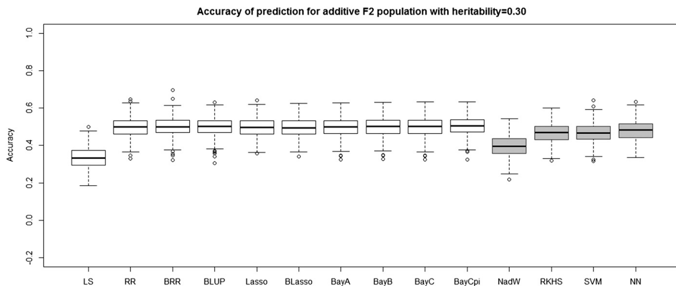
Figure 7 The boxplots of accuracy of prediction for the F_2 population with additive genetic architecture and heritability of 0.30. The first 10 boxplots correspond to the parametric methods, and the last four (gray) boxplots correspond to the nonparametric methods.
