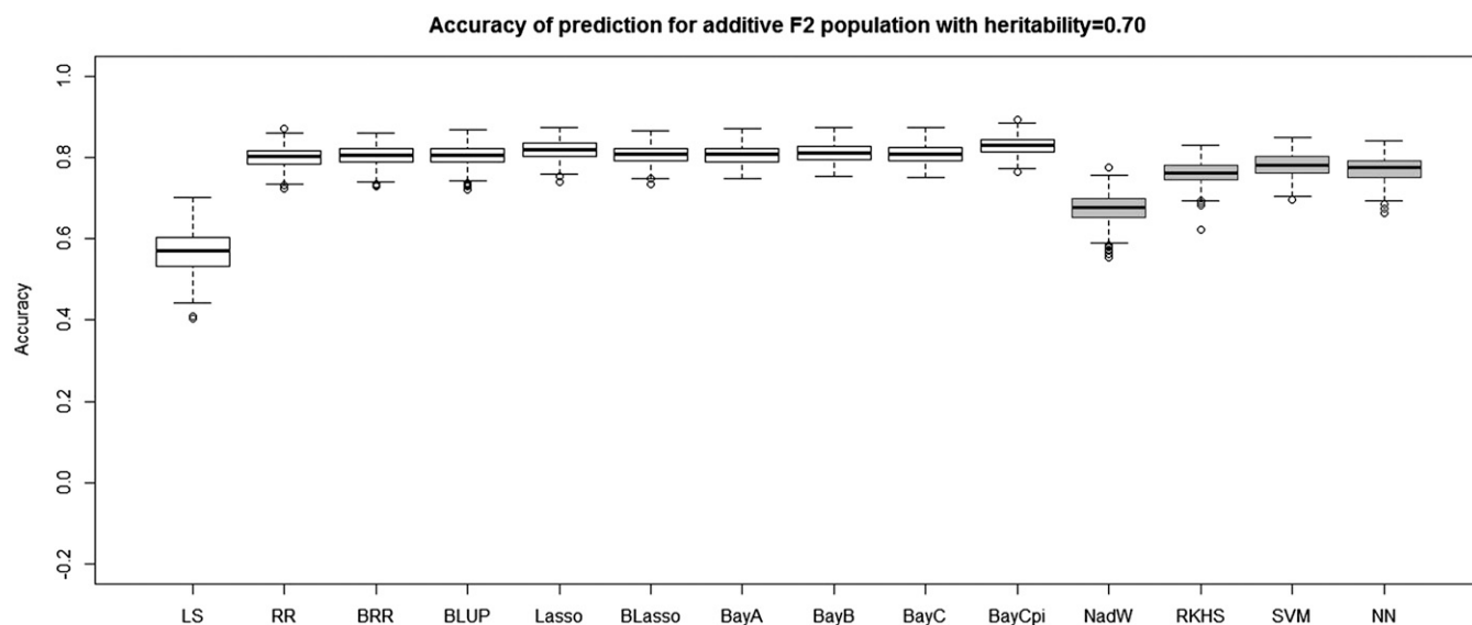
Figure 5 The boxplots of accuracy of prediction for the F_2 population with additive genetic architecture and heritability of 0.70. The first 10 boxplots correspond to the parametric methods, and the last four (gray) boxplots correspond to the nonparametric methods.
