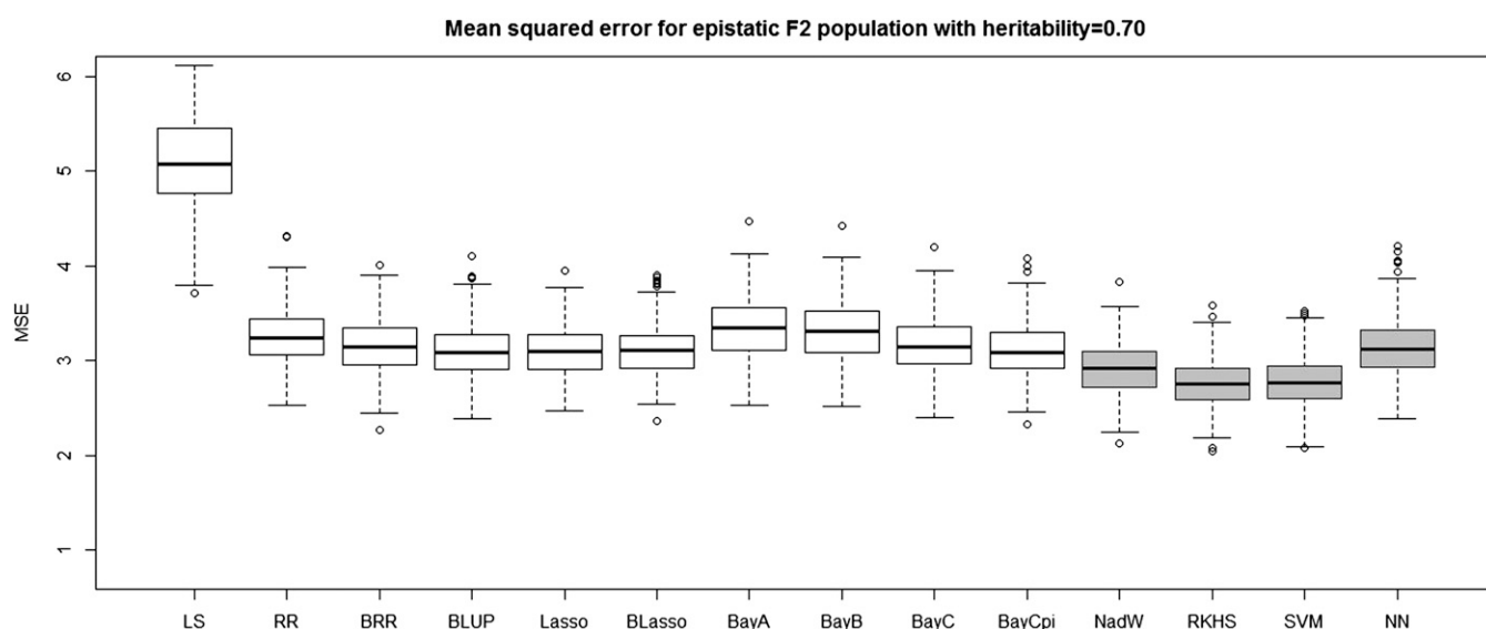
Figure 10 The boxplots of mean squared error for the F_2 population with epistatic genetic architecture and heritability of 0.70. The first 10 boxplots correspond to the parametric methods, and the last four (gray) boxplots correspond to the nonparametric methods.
