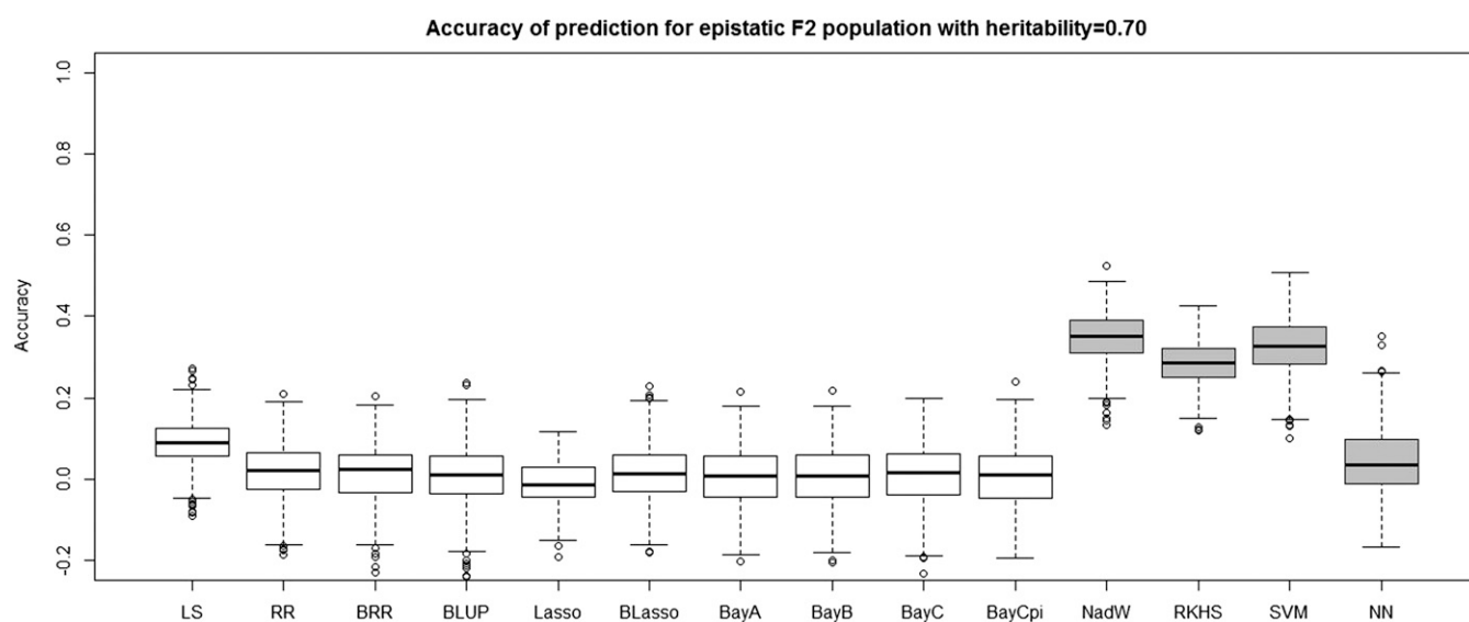
Figure 6 The boxplots of accuracy of prediction for the F_2 population with epistatic genetic architecture and heritability of 0.70. The first 10 boxplots correspond to the parametric methods, and the last four (gray) boxplots correspond to the nonparametric methods.
