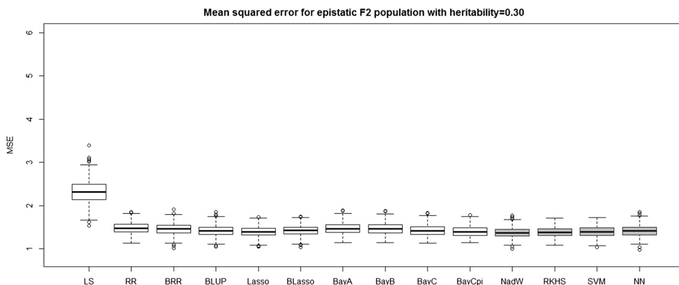
Figure 12 The boxplots of mean squared error for the F_2 population with epistatic genetic architecture and heritability of 0.30. The first 10 boxplots correspond to the parametric methods, and the last four (gray) boxplots correspond to the nonparametric methods.
